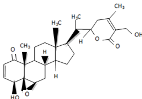
Fig 10. Structure of RA-1
