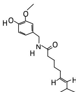
Fig 5.-Structure of Capsaicin
