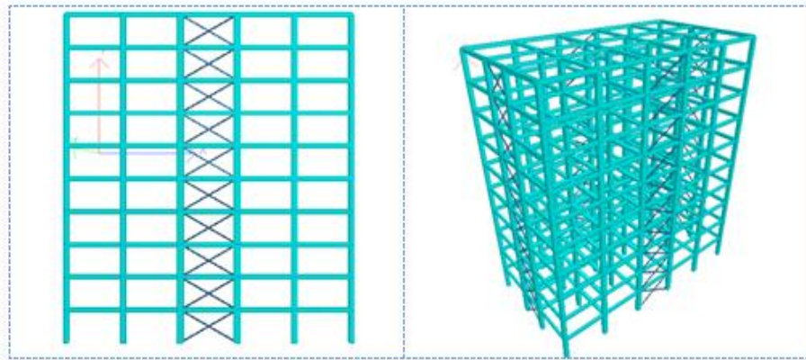
Fig. 5. Elevation & Isometric View of 10-Storey with Braced Frame
