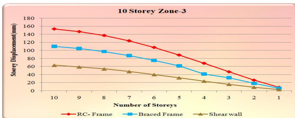
Graph 1. Storey Displacement Comparisons with RC-Frame (zone-3)
