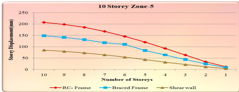
Graph 2. Storey Displacement Comparisons with RC-Frame (zone-5)
