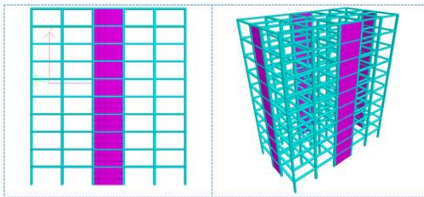
Fig. 6. Elevation & Isometric View of 10-Storey with Shear Wall
