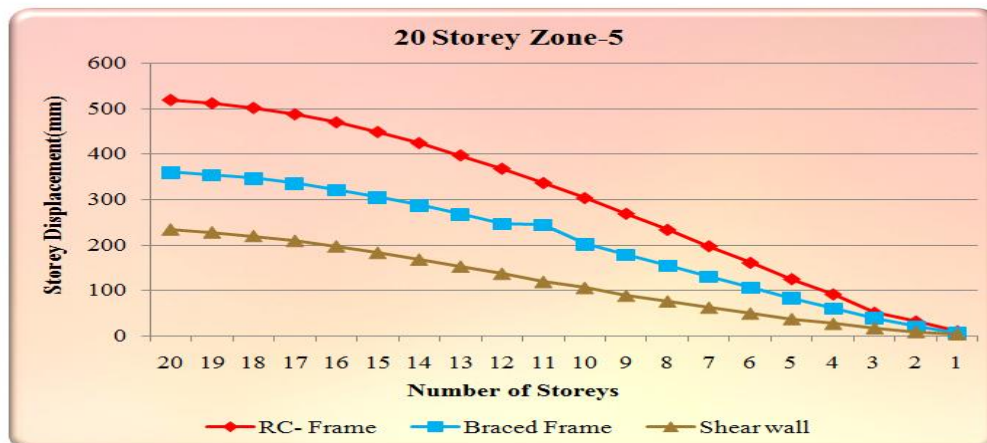
Graph 3.4: Storey Displacement Comparisons with RC-Frame (zone-5)
