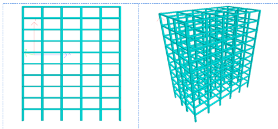
Fig. 4. Elevation & Isometric View of 10-Storey RC-Frame
