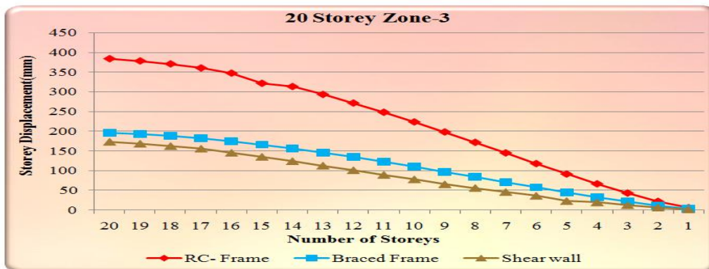
Graph 3.3: Storey Displacement Comparisons with RC-Frame (zone-3)
