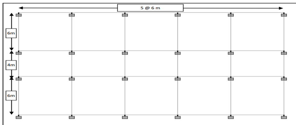
Fig 1. Plan of Model
